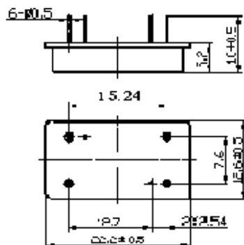
Package Outline
